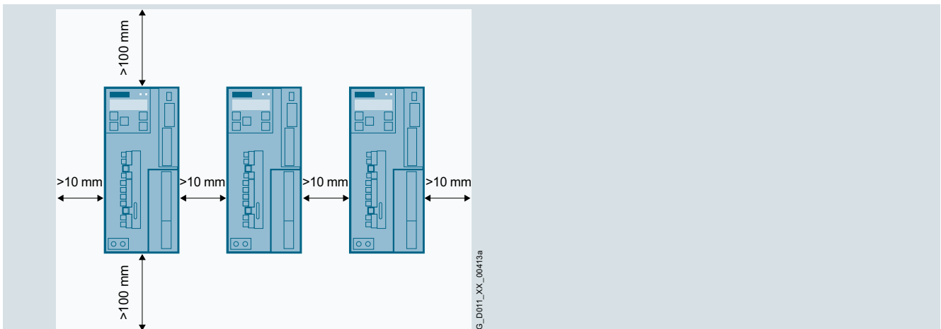
Mounting clearances
